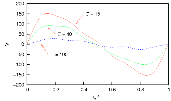
FIG. 3. Average velocity V of the cloud of particles as a function of the transition rates between internal states. V is plotted versus \gamma_+ for a fixed value of \Gamma = \gamma_+ + \gamma_- . Parameters of the simulation are A = 200 , D_v = 75 , and \phi = 3\pi/2 .
